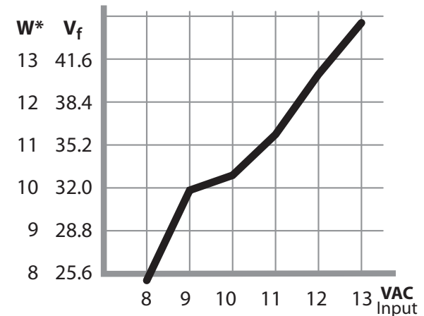
Voltage Input vs. Forward Voltage Output
